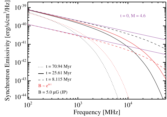
Figure 3. Left: time evolution of cooling CR spectra n(p, t) in cgs units. The standard JP model is shown in black with the time in Myr above the break. The linear and exponential models are shown as in green and red, respectively. Right: time evolution of synchrotron spectra of the standard and the exponential model (standard, black; exponential, red) at three different times, 8, t_{\text{eq}} and 83 Myr as dashed, full and dotted line, respectively. The injection is marked as purple line.
